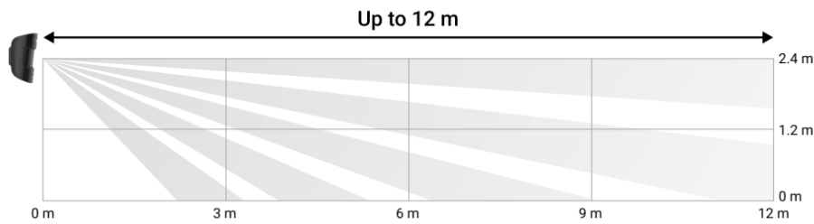
The vertical viewing angle of the detector
